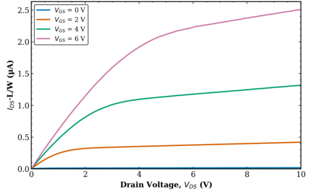
TFT3 Transistor 1 L = 160 \mu\text{m} - avg over all W (mean \pm std)
