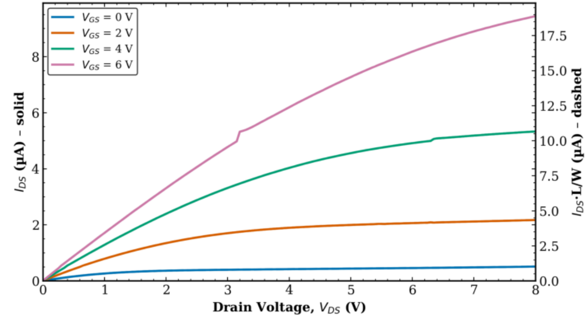
TFT3 Transistor 1 L = 20 \mu\text{m} , W = 10 \mu\text{m}
