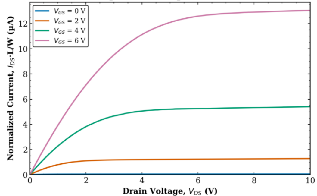
TFT3 Transistor 1 L = 40 \mu\text{m} , W = 50 \mu\text{m} (normalized)
