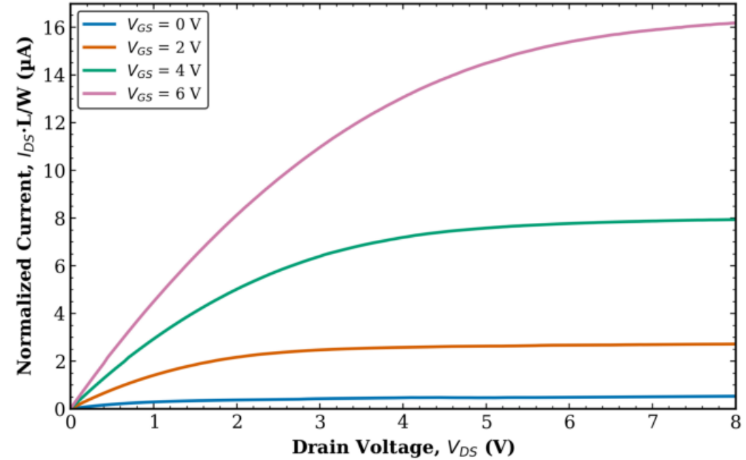
TFT3 Transistor 1 L = 20 \mu\text{m} , W = 50 \mu\text{m} (normalized)
