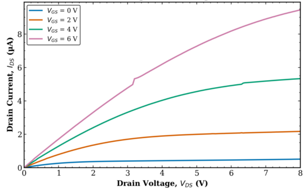
TFT3 Transistor 1 L = 20 \mu\text{m} , W = 10 \mu\text{m}
