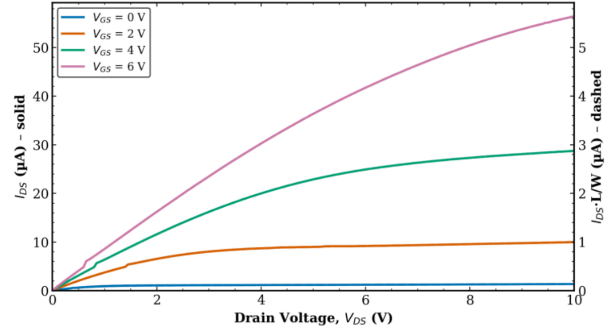
TFT3 Transistor 1 L = 10 \mu\text{m} , W = 100 \mu\text{m}
