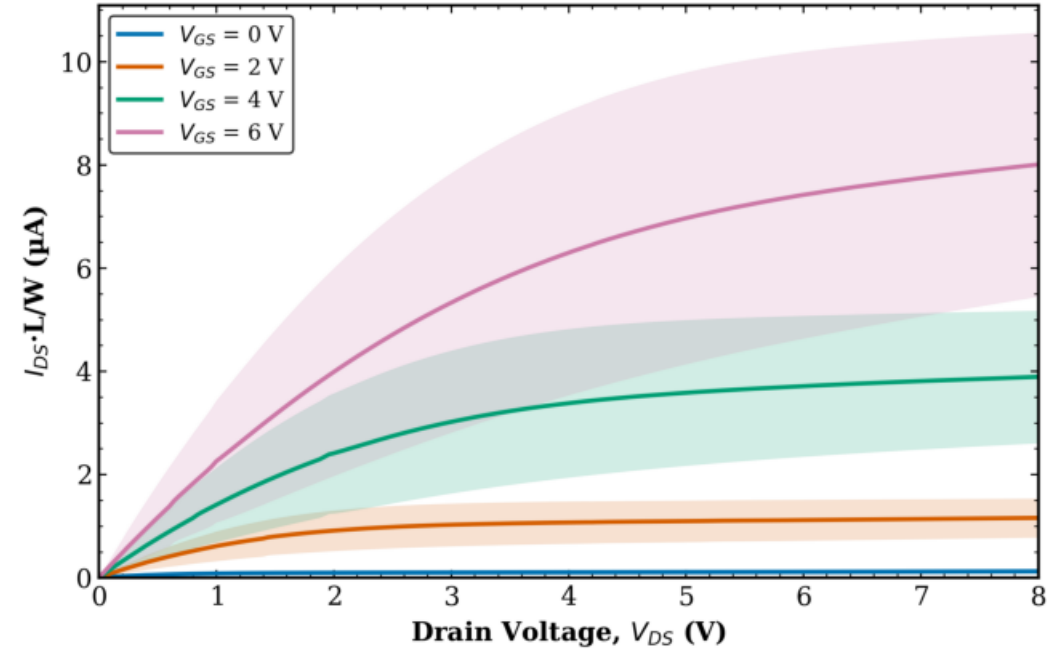
TFT3 Transistor 1 W = 100 \mu\text{m} - avg over all L (mean \pm std)
