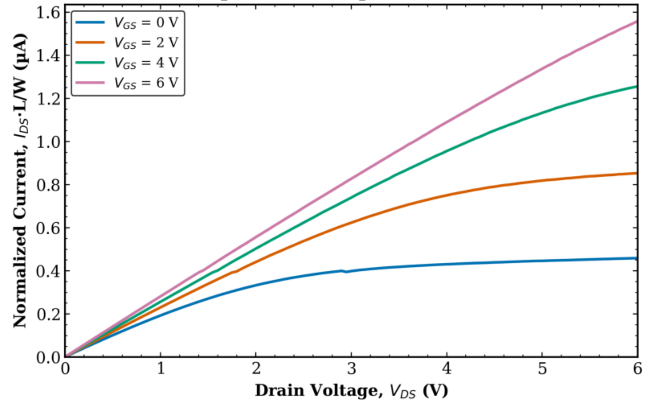
TFT3 Transistor 1 L = 8 \mu\text{m} , W = 10 \mu\text{m} (normalized)
