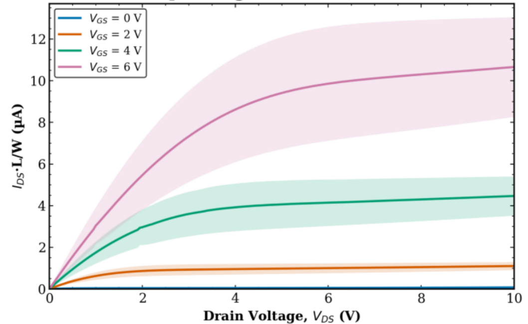
TFT3 Transistor 1 L = 40 \mu\text{m} - avg over all W (mean \pm std)
