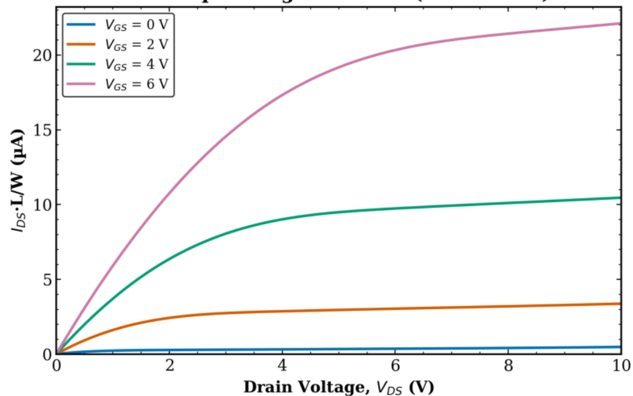
TFT3 Transistor 1 L = 80 \mu\text{m} - avg over all W (mean \pm std)
