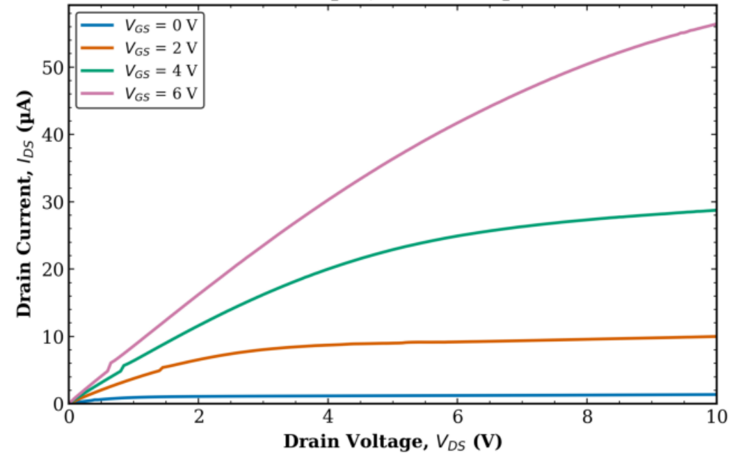
TFT3 Transistor 1 L = 10 \mu\text{m} , W = 100 \mu\text{m}
