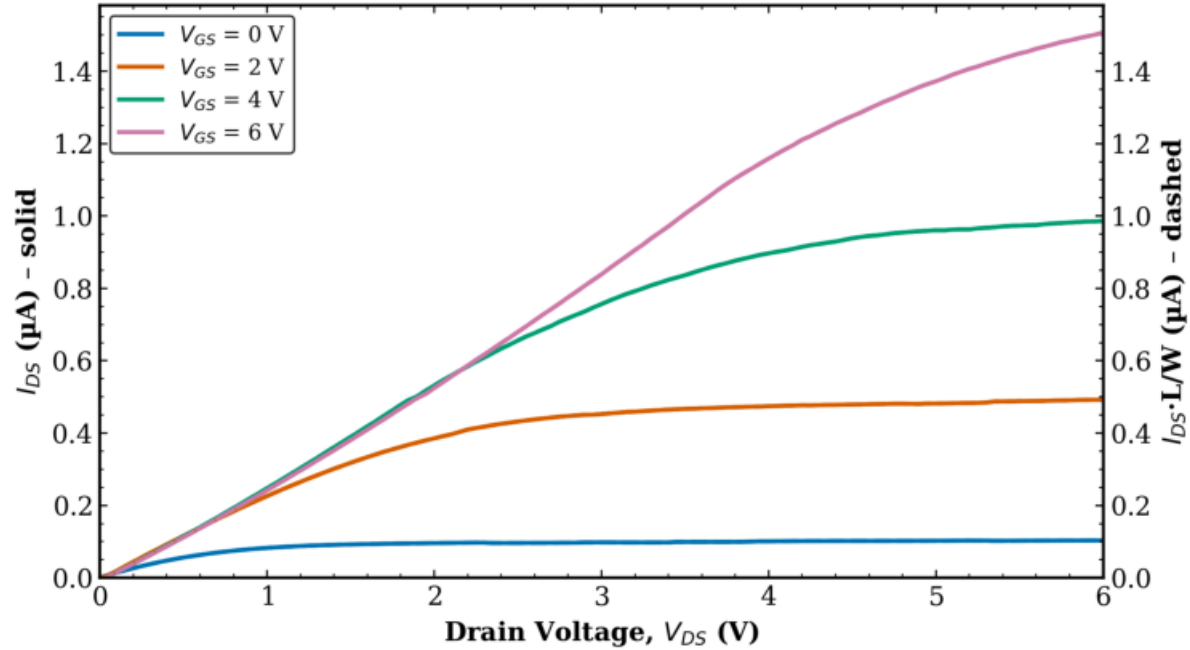
TFT3 Transistor 1 L = 10 \mu\text{m} , W = 10 \mu\text{m}
