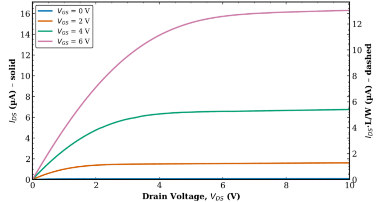
TFT3 Transistor 1 L = 40 \mu\text{m} , W = 50 \mu\text{m}
