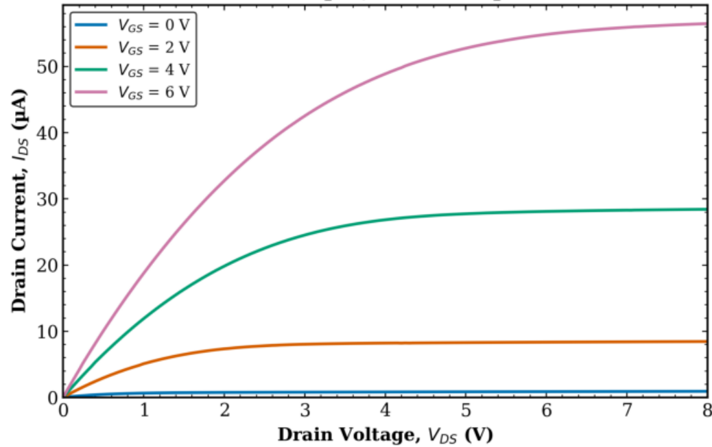
TFT3 Transistor 1 L = 20 \mu\text{m} , W = 100 \mu\text{m}
