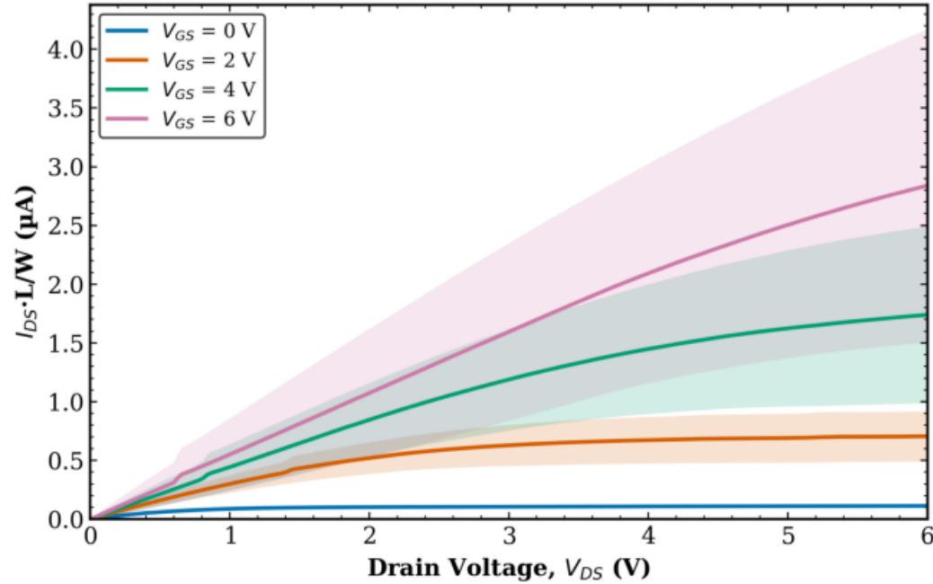
TFT3 Transistor 1 L = 10 \mu\text{m} - avg over all W (mean \pm std)
