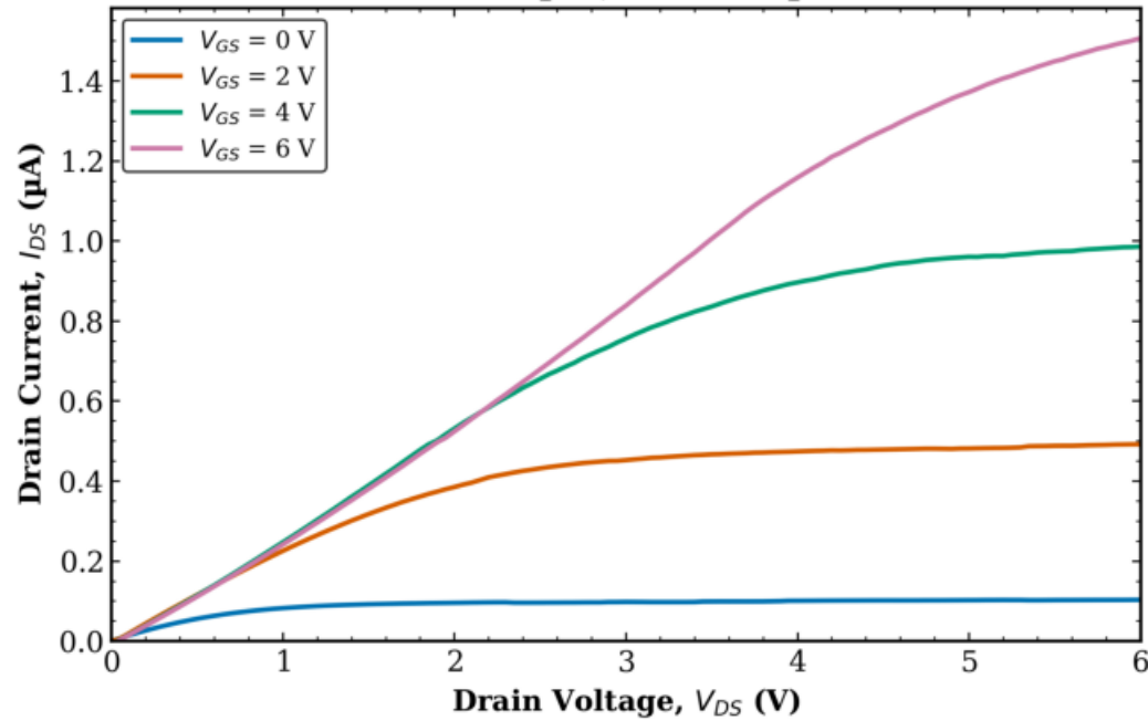
TFT3 Transistor 1 L = 10 \mu\text{m} , W = 10 \mu\text{m}
