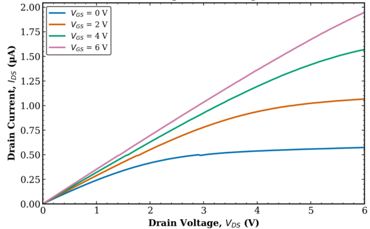
TFT3 Transistor 1 L = 8 \mu\text{m} , W = 10 \mu\text{m}
