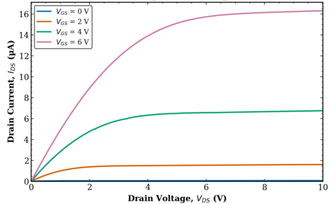
TFT3 Transistor 1 L = 40 \mu\text{m} , W = 50 \mu\text{m}
