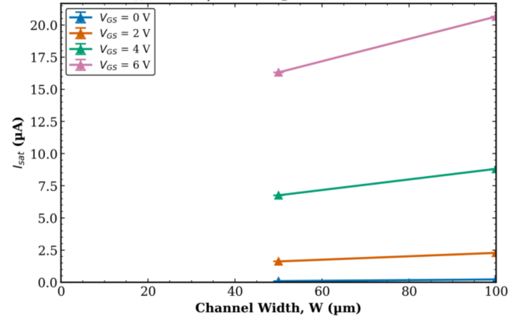
TFT3 Transistor 1 I_{sat} vs W | L = 40 μm (mean \pm std)
