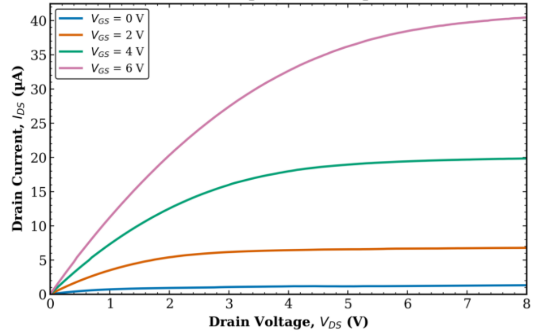
TFT3 Transistor 1 L = 20 \mu\text{m} , W = 50 \mu\text{m}
