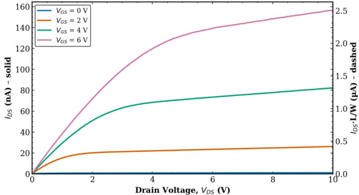
TFT3 Transistor 1 L = 160 \mu\text{m} , W = 10 \mu\text{m}
