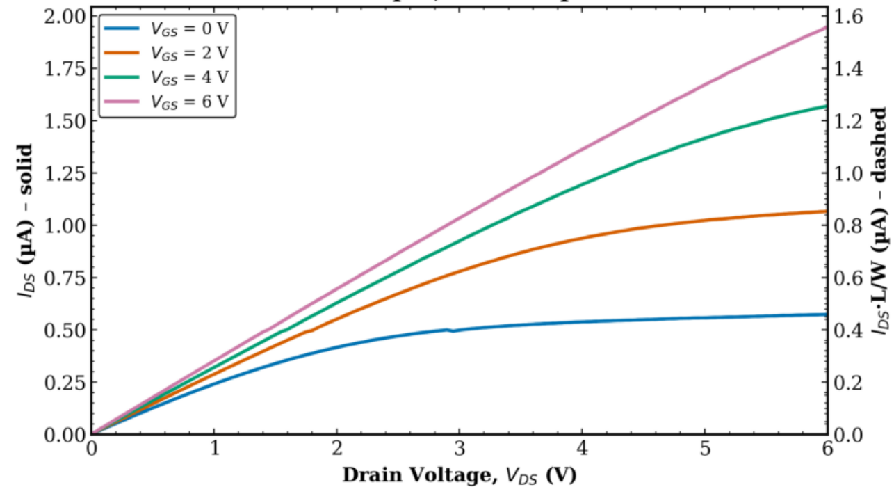
TFT3 Transistor 1 L = 8 \mu\text{m} , W = 10 \mu\text{m}
