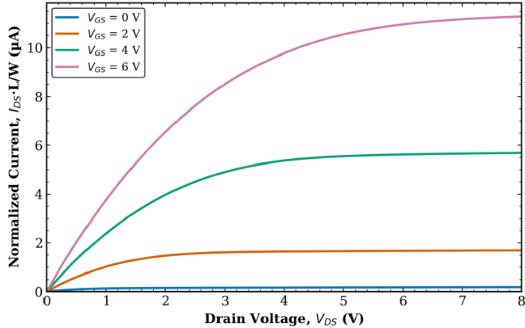
TFT3 Transistor 1 L = 20 \mu\text{m} , W = 100 \mu\text{m} (normalized)
