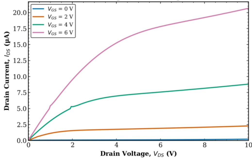
TFT3 Transistor 1 L = 40 \mu\text{m} , W = 100 \mu\text{m}
