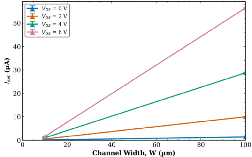
TFT3 Transistor 1 I_{sat} vs W | L = 10 \mu\text{m} (mean \pm std)
