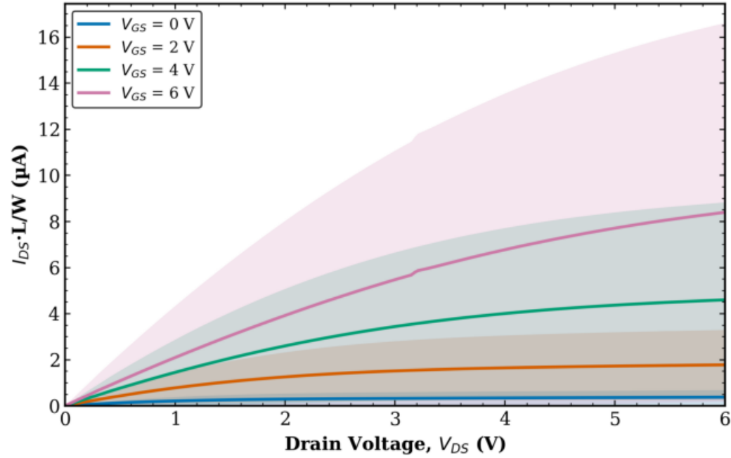
TFT3 Transistor 1 W = 10 \mu\text{m} - avg over all L (mean \pm std)
