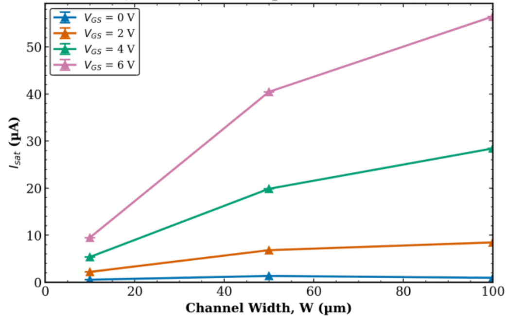
TFT3 Transistor 1 I_{sat} vs W | L = 20 μm (mean \pm std)
