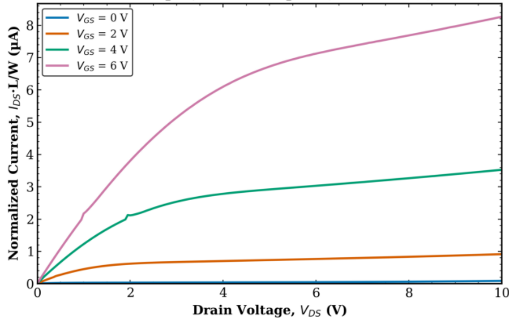
TFT3 Transistor 1 L = 40 \mu\text{m} , W = 100 \mu\text{m} (normalized)
