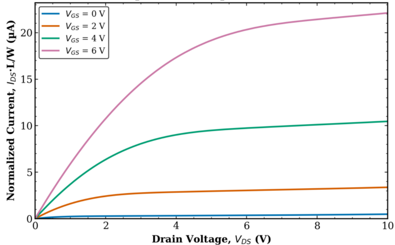
TFT3 Transistor 1 L = 80 \mu\text{m} , W = 10 \mu\text{m} (normalized)
