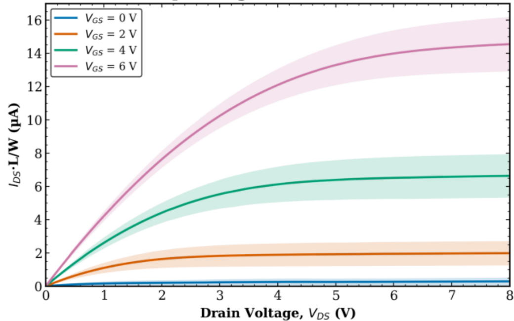
TFT3 Transistor 1 W = 50 \mu\text{m} - avg over all L (mean \pm std)
