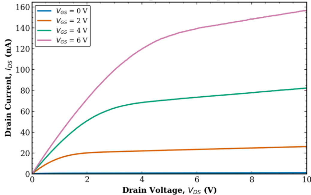
TFT3 Transistor 1 L = 160 \mu\text{m} , W = 10 \mu\text{m}
