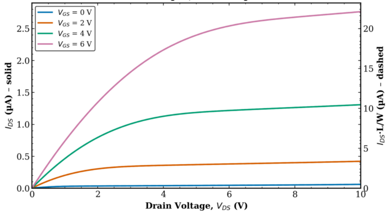
TFT3 Transistor 1 L = 80 \mu\text{m} , W = 10 \mu\text{m}
