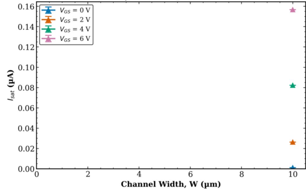
TFT3 Transistor 1 I_{sat} vs W | L = 160 μm (mean \pm std)
