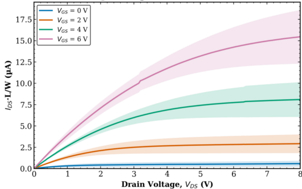
TFT3 Transistor 1 L = 20 \mu\text{m} - avg over all W (mean \pm std)
