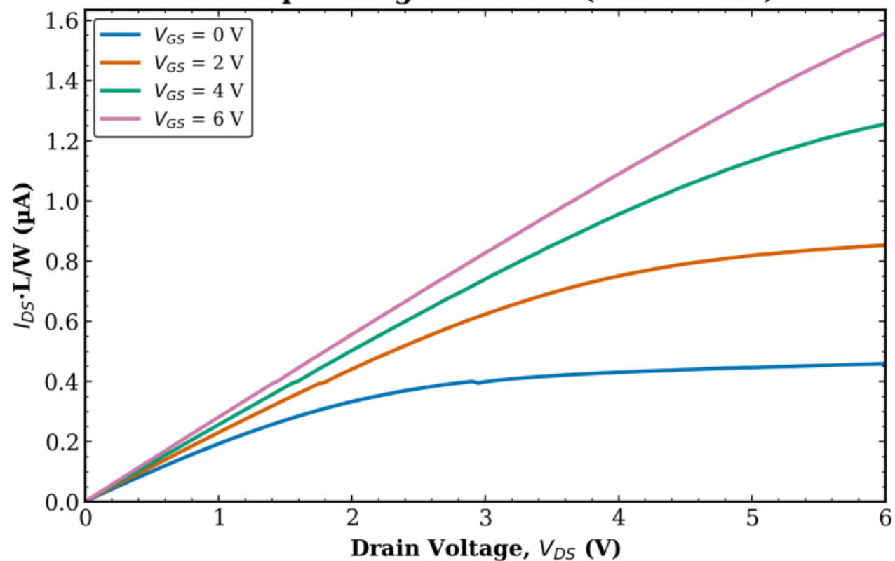
TFT3 Transistor 1 L = 8 \mu\text{m} - avg over all W (mean \pm std)
