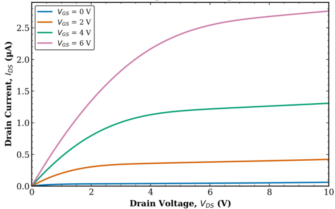
TFT3 Transistor 1 L = 80 \mu\text{m} , W = 10 \mu\text{m}
