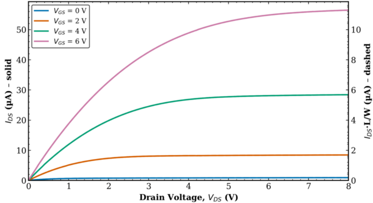
TFT3 Transistor 1 L = 20 \mu\text{m} , W = 100 \mu\text{m}
