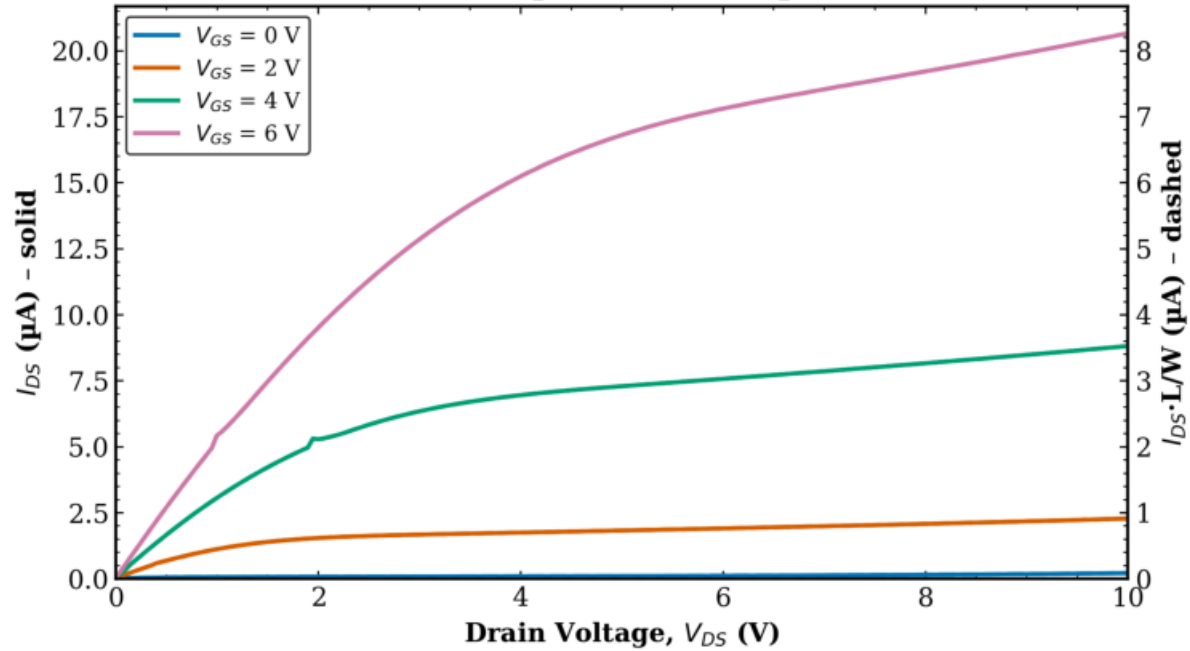
TFT3 Transistor 1 L = 40 \mu\text{m} , W = 100 \mu\text{m}
